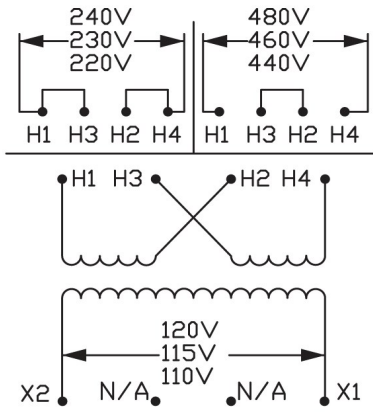
Wiring Diagram
